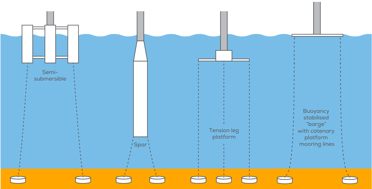
FIGURE 31 The four main technologies for floating offshore wind
