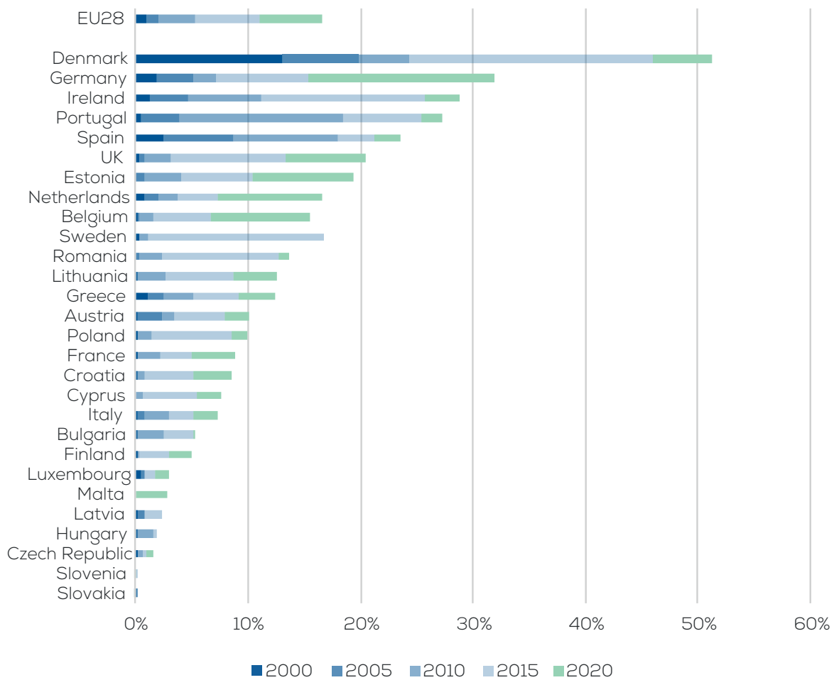
FIGURE 26 Evolution of wind energy share in EU’s electricity demand
