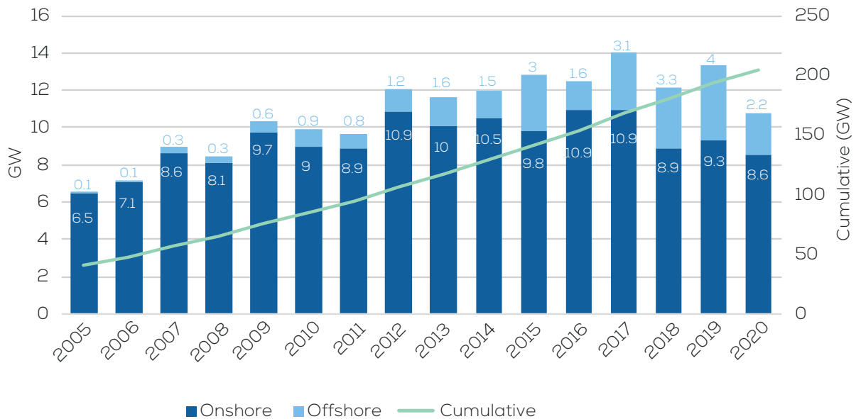
FIGURE 17 Wind energy market outlook in the EU28 under WindEurope's Central Scenario
