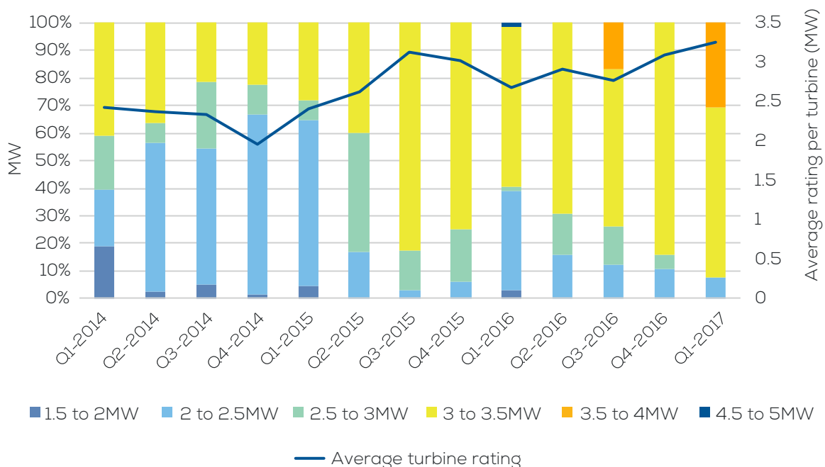
FIGURE 27 Capacity rating of ordered onshore wind turbines in Europe
