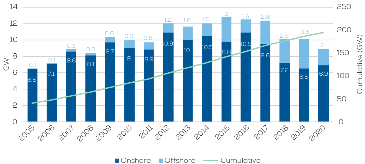
FIGURE 20 Annual and cumulative installations under WindEurope’s Low Scenario
