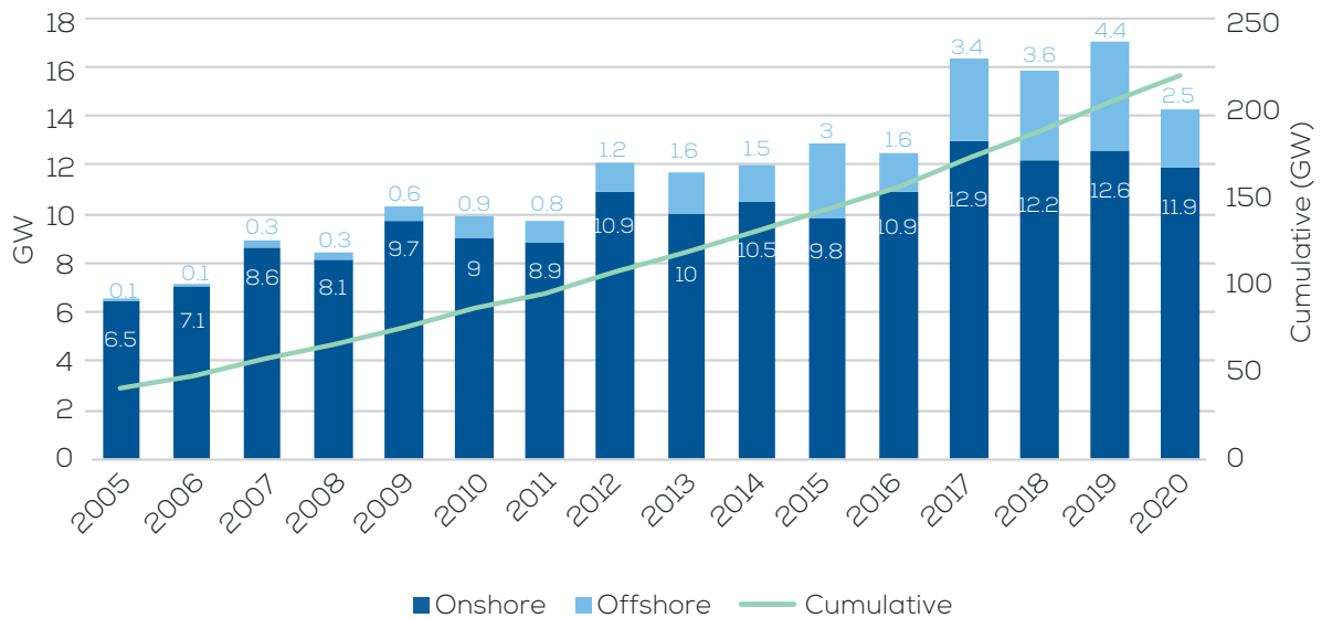
FIGURE 21 Market and cumulative installations under WindEurope’s High Scenario
