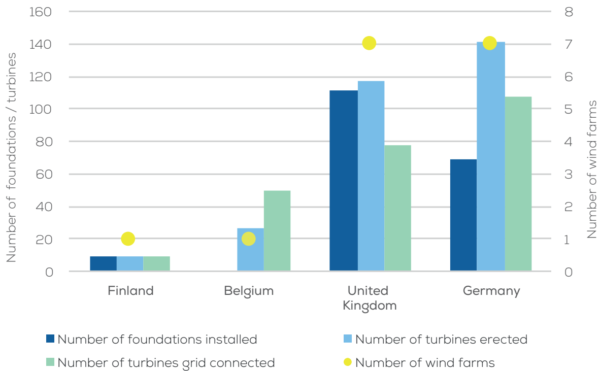
FIGURE 5 Summary of work in offshore wind farms between 1 st January and 30 th June 2017
