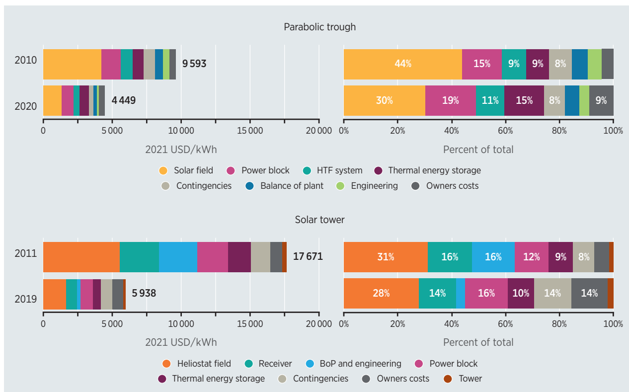
Figure 5.2 Total installed cost breakdown of CSP plants by technology (2010/2011 and 2019/2020)
