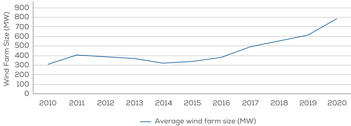
FIGURE 7 Average size of commercial offshore wind farm projects in the year (MW)
